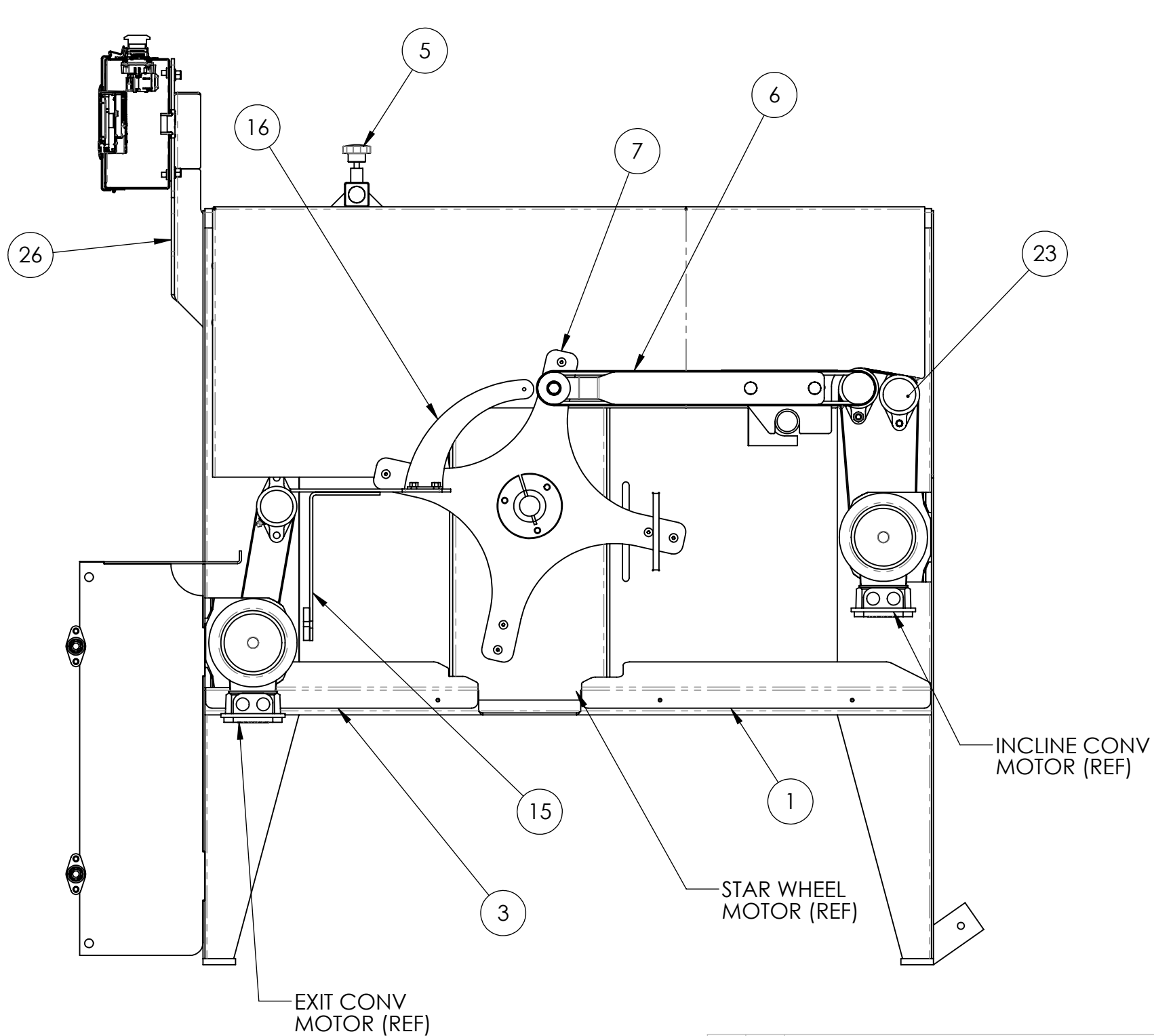
SECTION F-F
